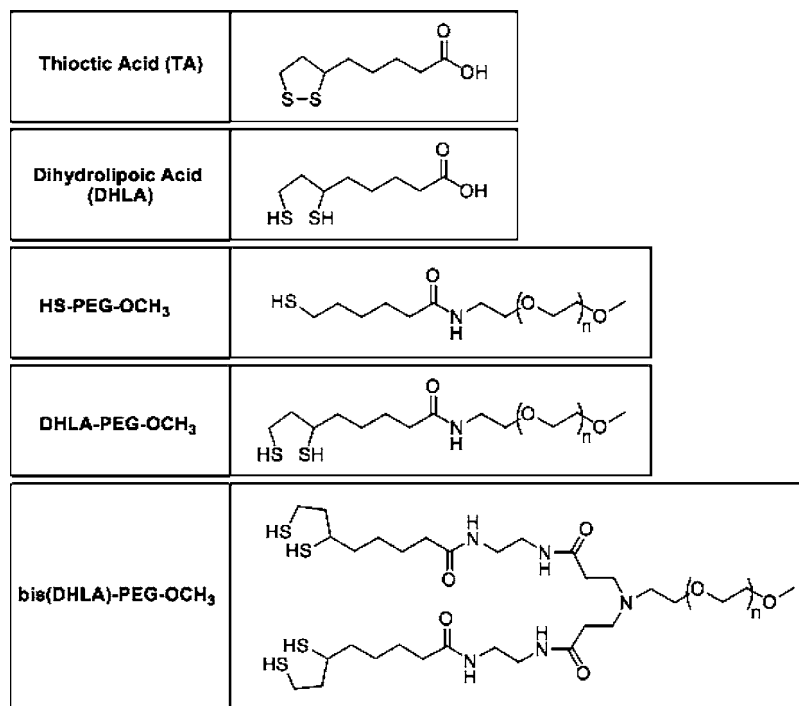
Figure 1. Structure of the PEG-appended ligands together with the disulfide precursor (PEG750 chain with n \approx 15 ). Only the reduced forms of the PEGylated ligands are shown.
